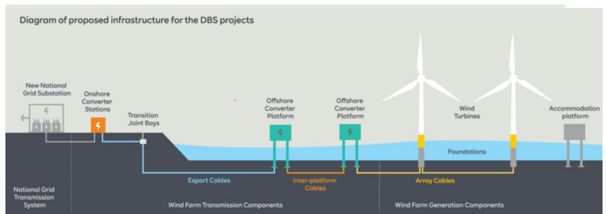
Plate 1-34 DBS East and DBS West Overview Schematic (N.B. Not to Scale)
